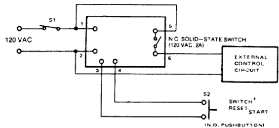
Vibraswitch with Monitor Delay or Start and Monitor Delay (Model 375A/376A-A2-XX or 375A/376A-A3-XX)
