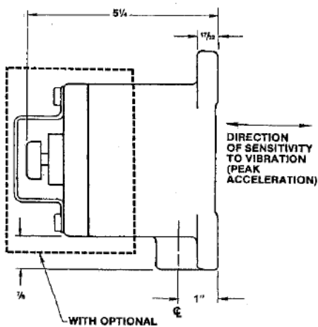
Figure 2a - Mounting dimensions for the Vibraswitch Model 375A
