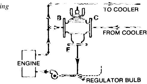
Figure 3: This drawing shows a method of controlling the cooling of engine lubricating oil.
