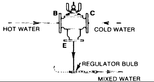
Figure 1: Illustrating a simple means for mixing hot and cold water where a rough mixing is suitable.
