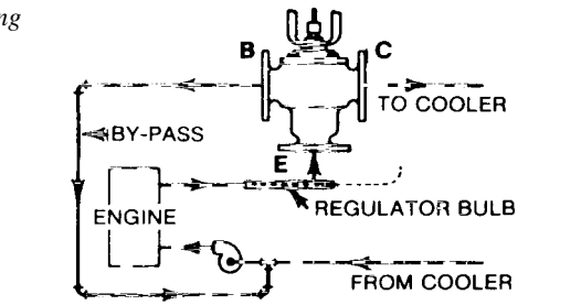
Figure 2: This drawing illustrates the most widely used method of cooling water control for internal combustion engines.
